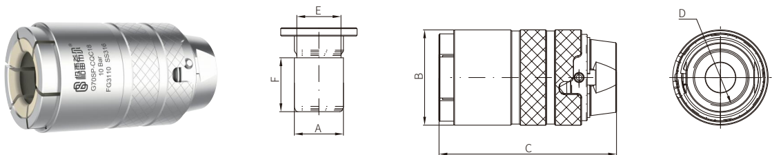
G70SP-CQC Damage-Free Small-Body Connector
