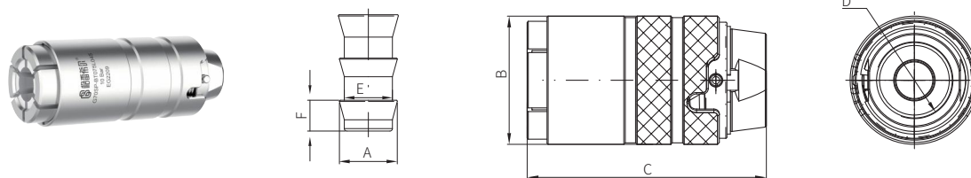
G70SP-BT Liquid Cooling Barbed Port
